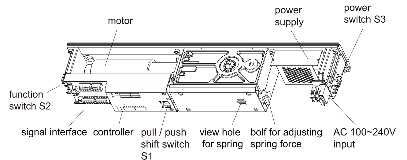
Drive device
