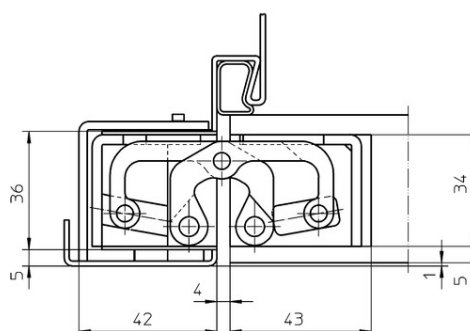
steel frame
