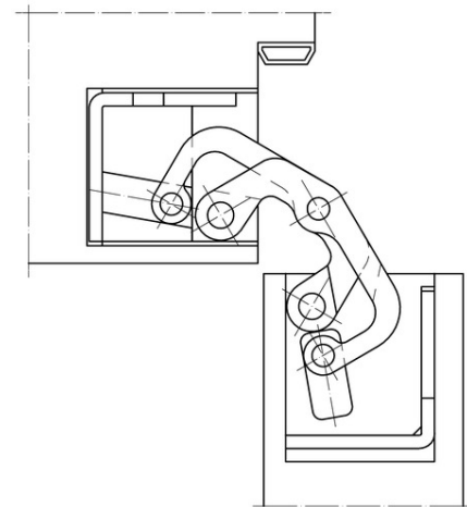
block frame 90°
