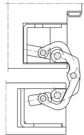
block frame 180°
