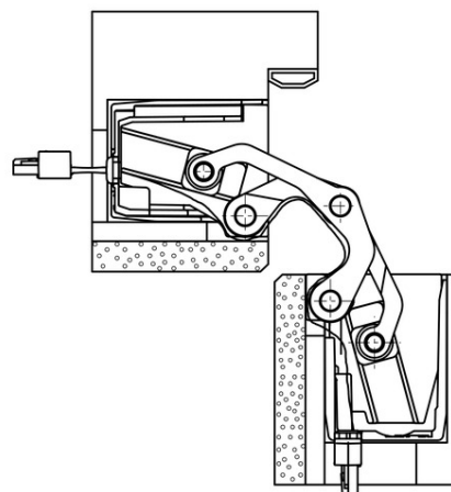
block frame 90°
