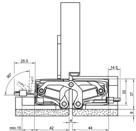
casing frame
