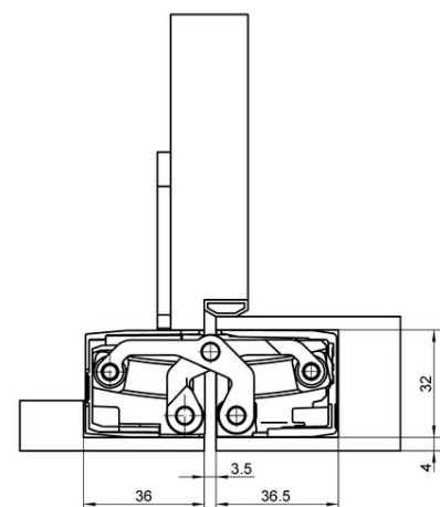
casing frame
