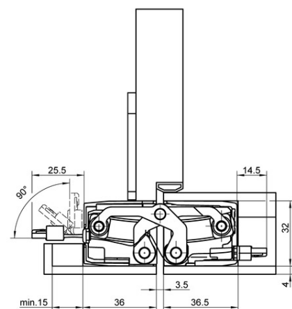
casing frame
