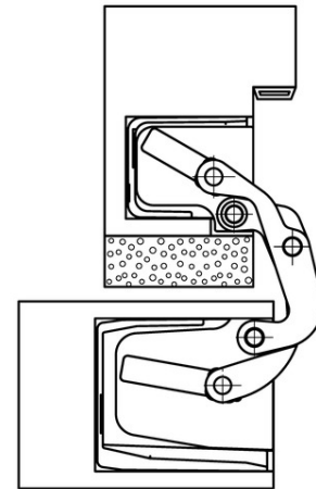
recessed frame facings 180°
