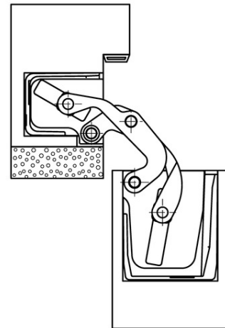
recessed frame facings 90°
