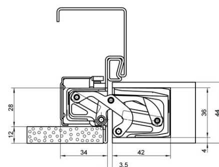
recessed steel frame facings
