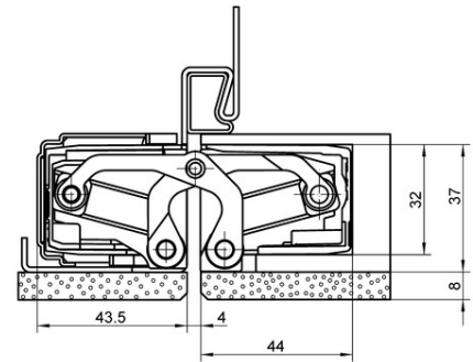
steel frame
