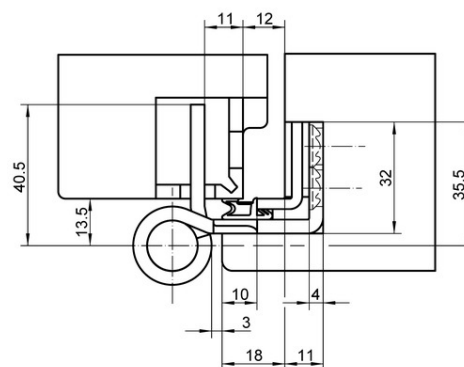
overlap 18 mm (finial 10)
