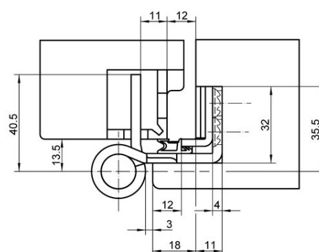
overlap 18 mm (finial 12)
