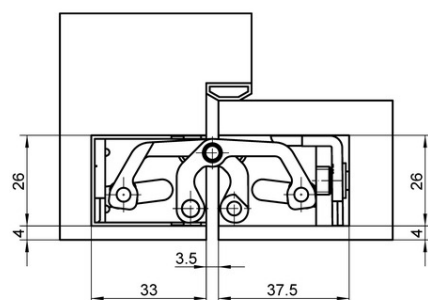
block frame
