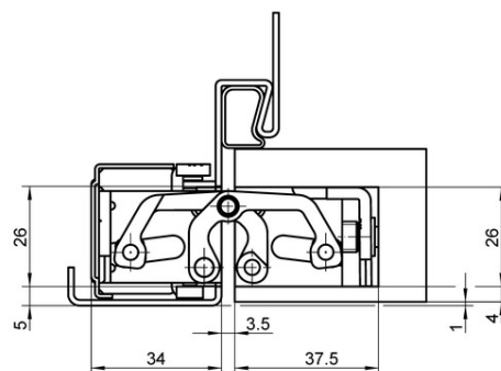
steel frame
