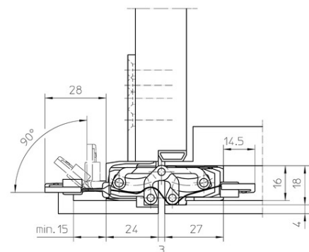
casing frame
